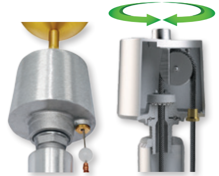
Internal Revolving - Spindle Design
