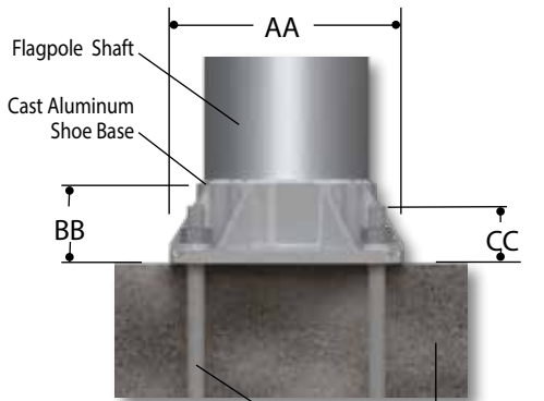
Four galvanized Steel Anchor Bolts (55,000 PSI Minimum Yield), 3000 PSI Concrete All Shoe Base Flagpoles are heat treated after weld to T-6 temper.
